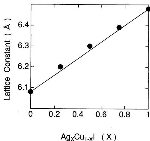
Fig. 2. The unit cell dimension of \text{Ag}_x\text{Cu}_{1-x}\text{I} crystal versus x = 0.0, 0.25, 0.50, 0.75, \text{ and } 1.0 ; The solid line is the Vegard law.
