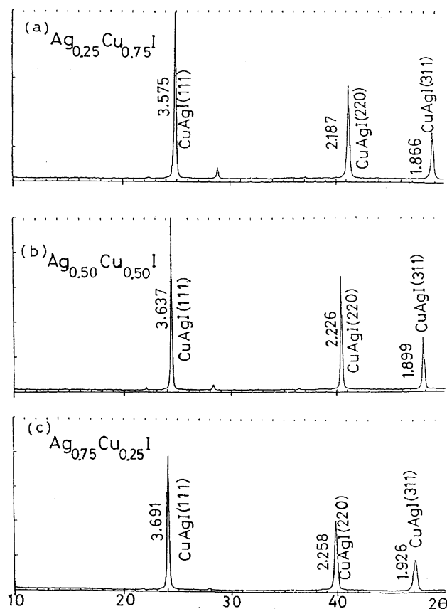
Fig. 1. X-Ray diffraction profiles of \text{Ag}_x\text{Cu}_{1-x}\text{I} crystal for x = 0.25, 0.5, \text{ and } 0.75 .
