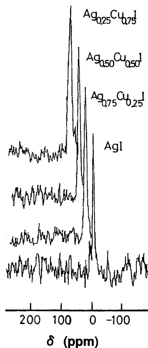
Fig. 3. ^{109}\text{Ag} MAS NMR spectra of \text{Ag}_x\text{Cu}_{1-x}\text{I} crystal for x = 0.25, 0.5, 0.75, \text{ and } 1.0 .
